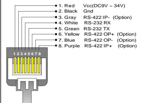
PMA-248 Pin Assignment
